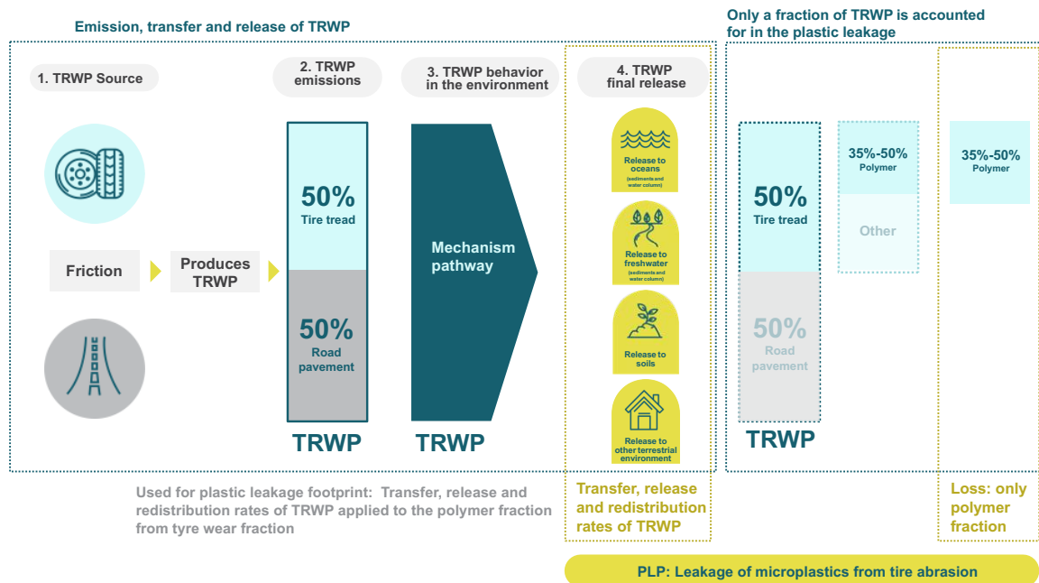
Figure 8.1: Tire and Road Wear Particles (TRWP) and calculation of leakage of microplastics from tire abrasion; the behavior of TRWP (i.e. the transfer, release and redistribution) is considered, but applied only to the theoretical fraction of polymer from tire fraction of TRWP
