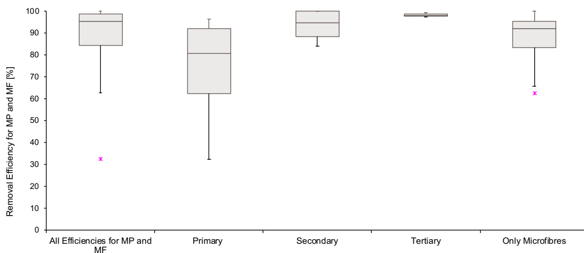
Figure 13.1: Removal efficiency for different levels of waste water treatment (primary, secondary and tertiary)
